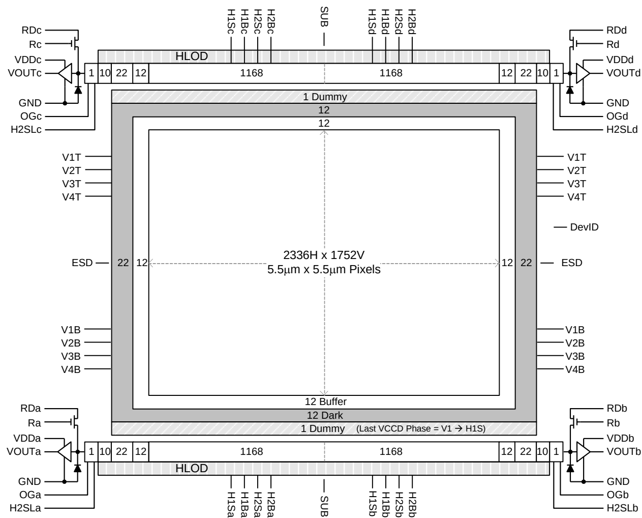
Figure 1: Block Diagram
