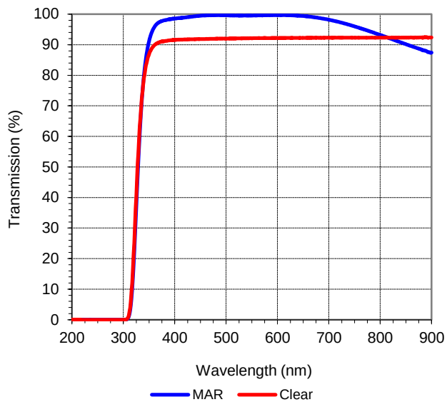
Figure 27: Cover Glass Transmission
