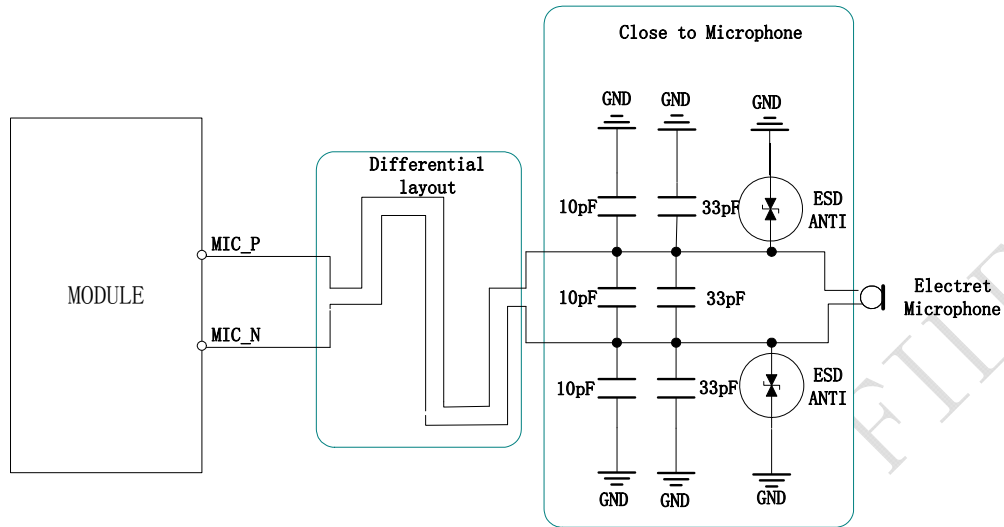
Figure 25: Microphone interface configuration
