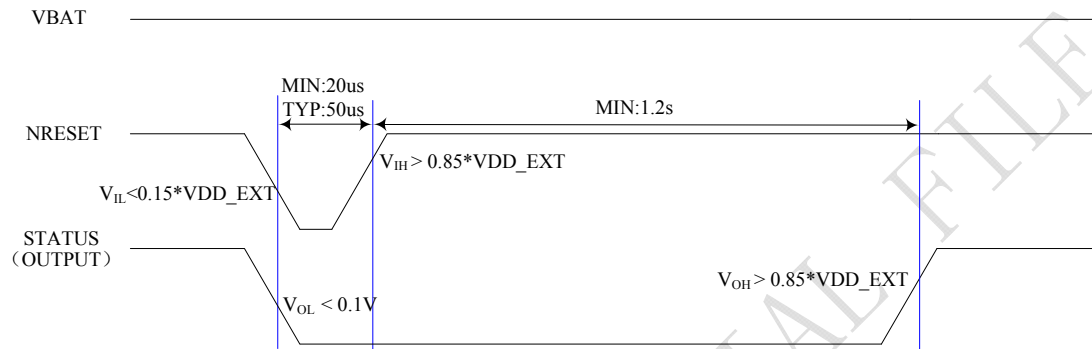
Figure 36: Reset timing
