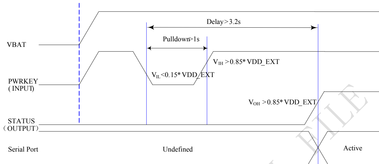
Figure 8: Timing of turn on system using PWRKEY
