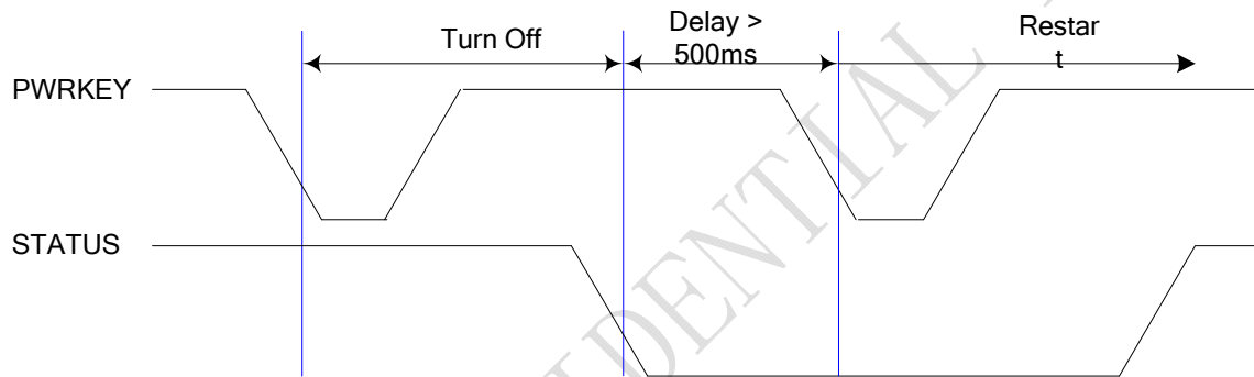
Figure 14: Timing of restart system
