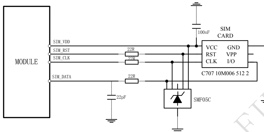
Figure 28: Reference circuit of the 6 pins SIM card
