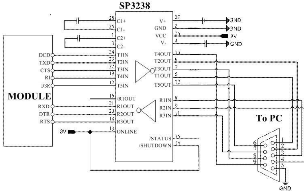
Figure 22: RS232 level converter circuit
