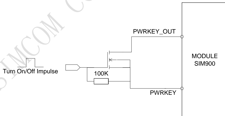
Figure 9: Turn on SIM900 using driving circuit
