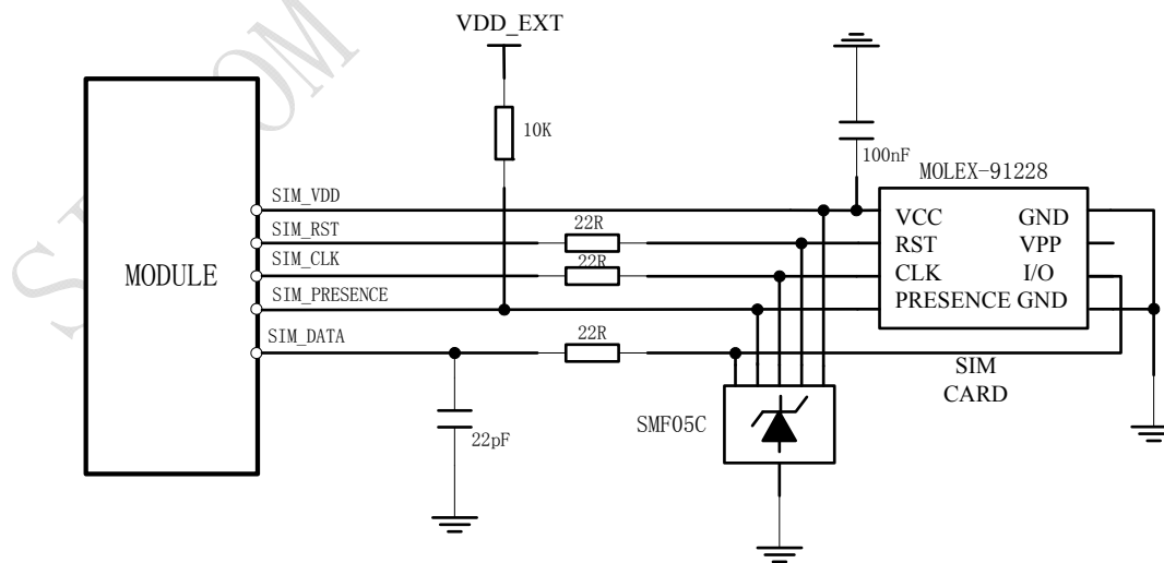
Figure 27: Reference circuit of the 8 pins SIM card
