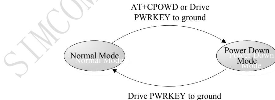
Figure 15: State Transition
