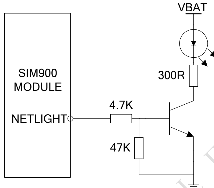
Figure 35: Reference circuit of NETLIGHT
