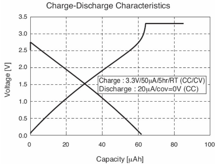
Figure 19: Seiko XH414H-IV01E Charge Characteristic
