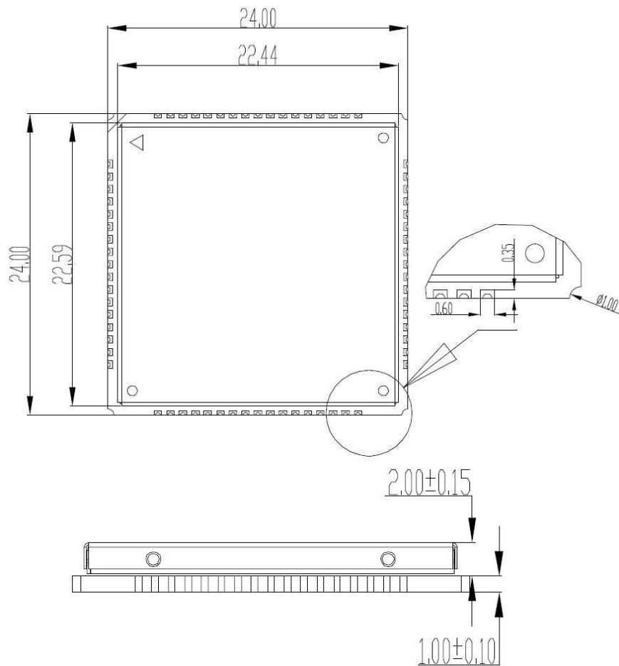
Figure 37: Top and Side Mechanical dimensions of module (Unit: mm)
