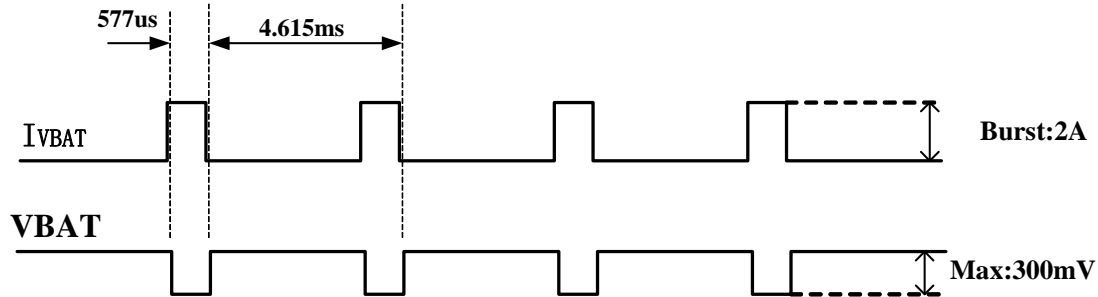
Figure 5: VBAT voltage drop during transmit burst
