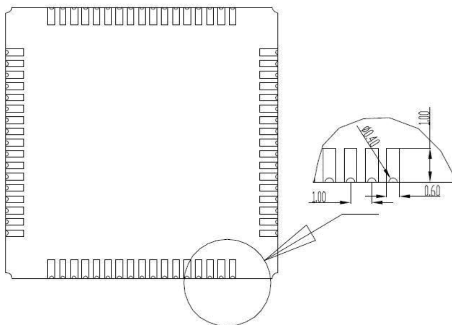
Figure 37: Top and Side Mechanical dimensions of module (Unit: mm)
