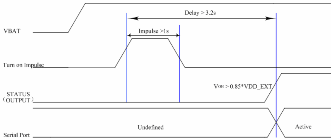
Figure 11: Timing of turn on system using PWRKEY and PWRKEY_OUT
