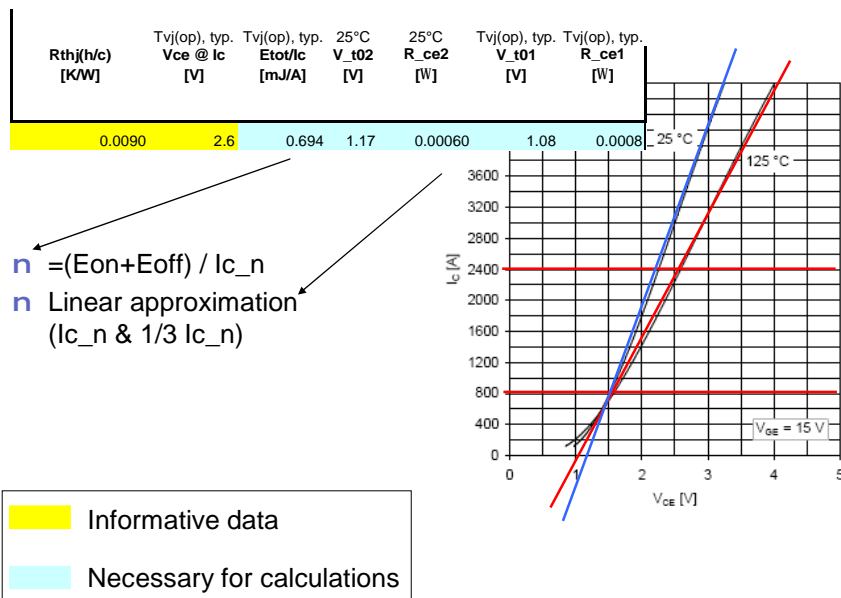
Fig. 40 Input fields for the IGBT loss characteristics.
