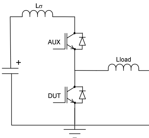
Fig. 6 Test circuit for the dynamic performance of the Diode
