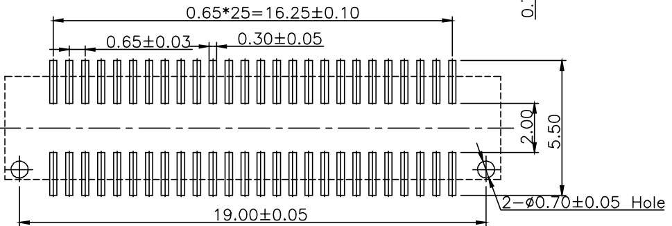
PCB LAYOUT
