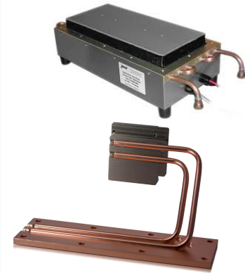
Custom Liquid Cold Plate Assemblies
