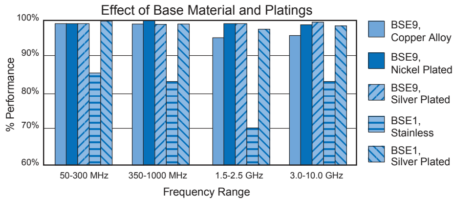
Figure 10. Springs made from stainless steel and copper alloy base materials were plated with nickel and silver. This graph shows their effect on transfer impedance (ZT) measurements.
