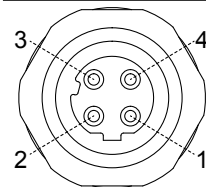
Connector M12 (female) 4-pin, D-coded
