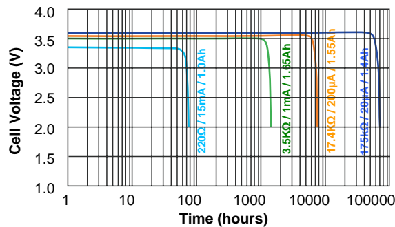
Typical discharge profile at 25°C
