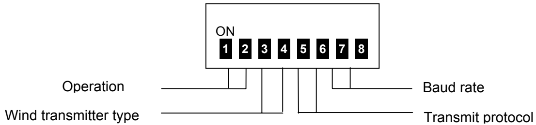
Figure 5: DIP-switch
