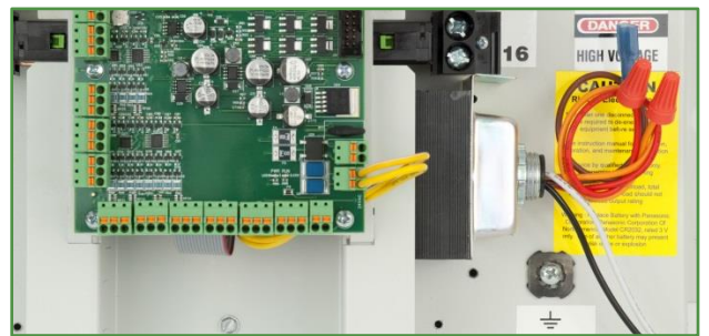
5. Replace CMP assembly and reconnect transformer secondary leads to CB (polarity of secondary leads is not specific). Reconnect transformer primary leads (common and power).
