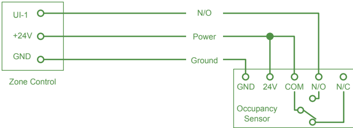
Universal Input DI Configuration (4-Wire 24V Occupancy Sensor)
