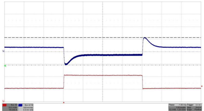
Fig. 22: Output voltage response to load current step change 50% - 100%-50% (21A–42A–21A) with di/dt = 1A/\mu s . Top trace (C4): Output voltage, Bottom trace (C3): Load current.
