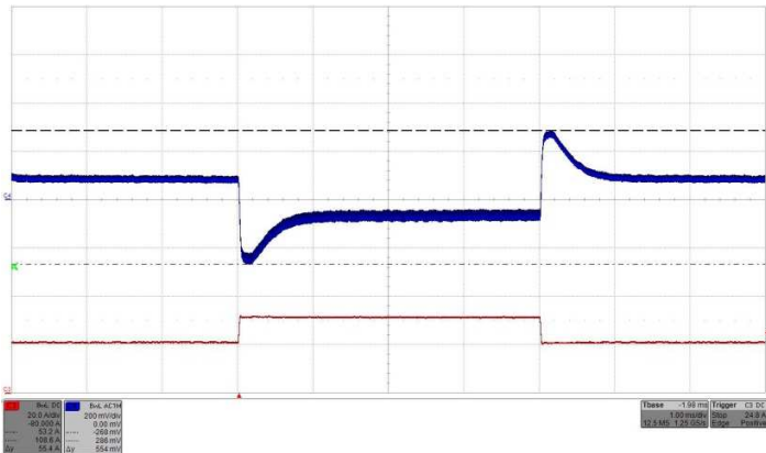
Fig. 21: Output voltage response to load current step change 50% - 75%-50% (21A–31.5A–21A) with di/dt = 1A/\mu s . Top trace (C4): Output voltage, Bottom trace (C3): Load current.
