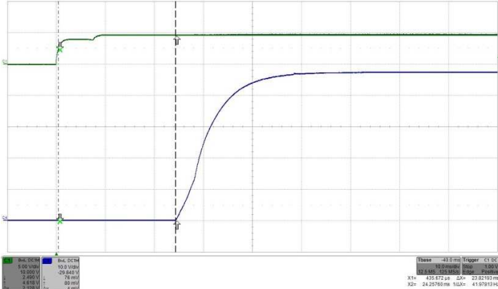
Fig. 31: Turn-on by ON/OFF transient ( V_{in} applied) at full rated load current (resistive). Top trace (C1): ON/OFF signal, Bottom trace (C4): Output voltage.
