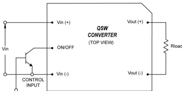
Fig 1: Circuit configuration for ON/OFF function.
