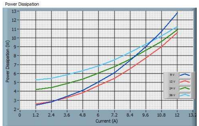
Fig. 5: Power Dissipation
