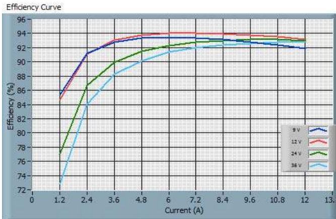
Fig. 4: Efficiency Curve
