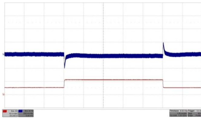
Fig. 9: Output voltage response to load current step change 50% - 100% - 50% (6A - 12A - 6A) with di/dt = 1A/\mu s at V_{IN} = 24V . Top trace (C4): Output voltage (200 mV/div.). Bottom trace (C3): Load current (10A/div.). C_O 330 \mu F/75m\Omega . Time: 1ms/div.
