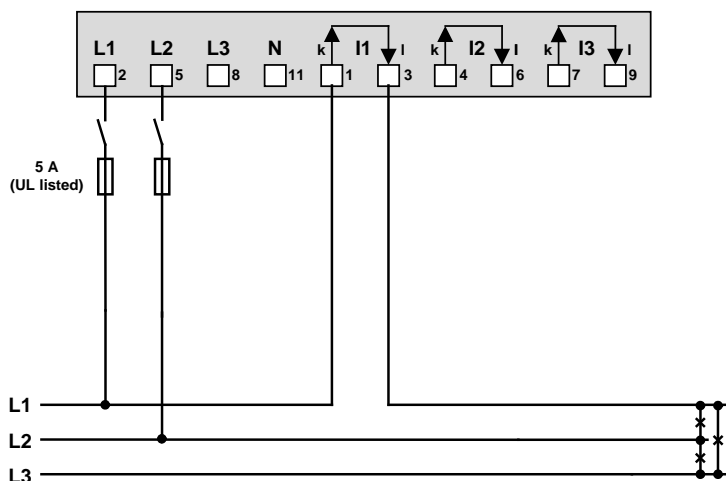
Direct connection
