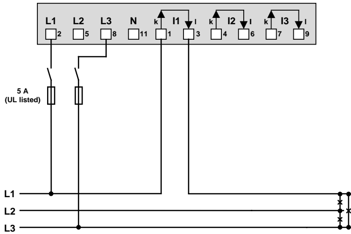
Direct connection
