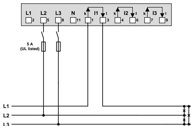
Direct connection
