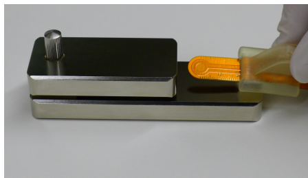
Figure 1: Metal to metal gap standard
