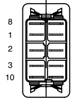
BOTTOM VIEW TERMINAL ARRANGEMENT 10 TERMINAL BASE
