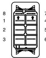
BOTTOM VIEW TERMINAL ARRANGEMENT 8 TERMINAL BASE
