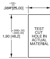
VMS MOUNTING PANEL HOLE
