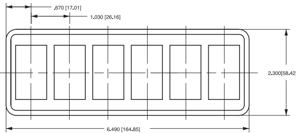
VM6 MOUNTING PANEL
