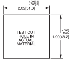
MOUNTING PANEL OPENING (2) UNITS
