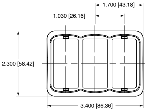
PANEL OPENING SIZE: 1.90 X 3.06 [48.3mm X 77.7mm]
