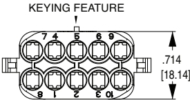
WCH CONNECTOR (190-31214-001)
