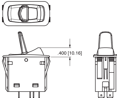
L-SERIES SHOWN WITH LARGE LENS AND PADDLE ACTUATOR
