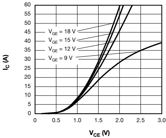
Fig. 19 - Typical Q2 - Q3 Trench IGBT 600 V Output Characteristics T_J = 125^\circ\text{C}
