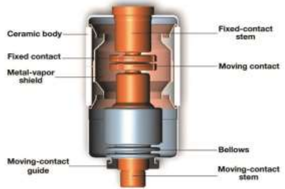
Figure 2. Internal view of a typical vacuum interrupter
