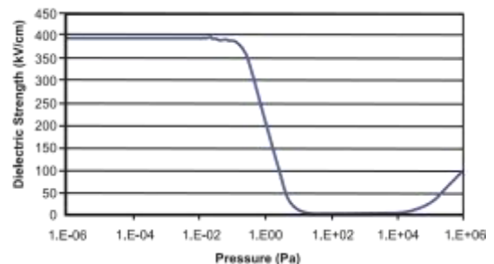
Figure 3. Paschen's curve for dry air
