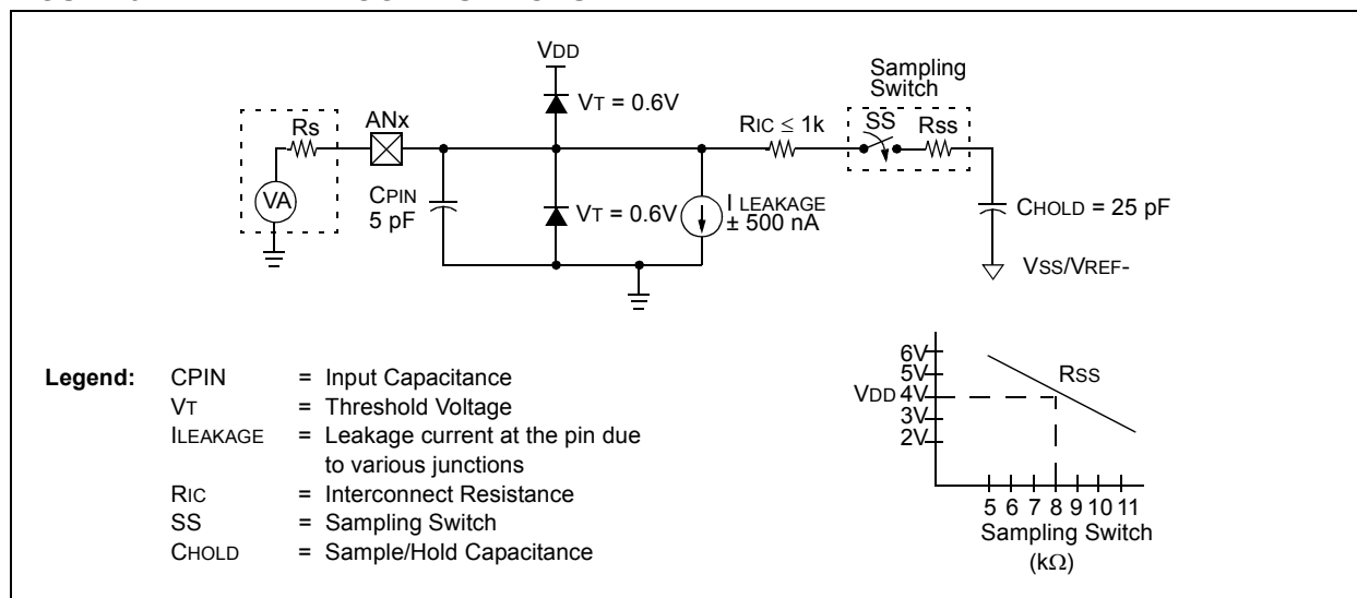
FIGURE 9-1: ANALOG INPUT MODULE
