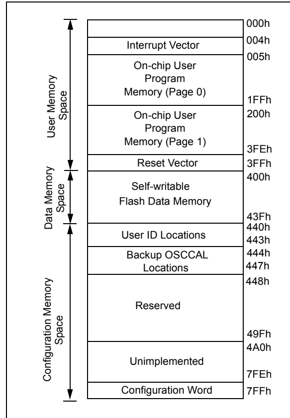
FIGURE 4-1: MEMORY MAP
