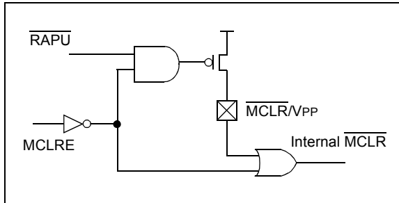
FIGURE 8-6: \overline{\text{MCLR}} SELECT
