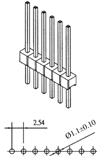
PC Board Layout
