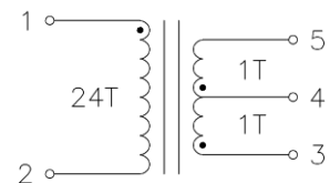
TP32D2402 (Full Bridge)
