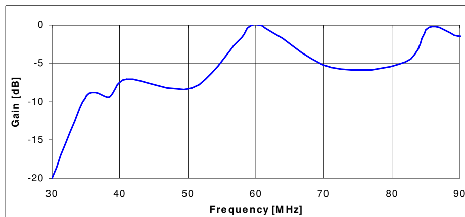
GAIN, relative \frac{1}{4}\lambda whip on GP
