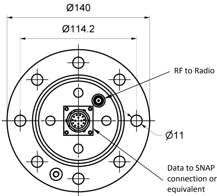
RF Connector: BNC Female Data Connector: PT02A-14-15P
