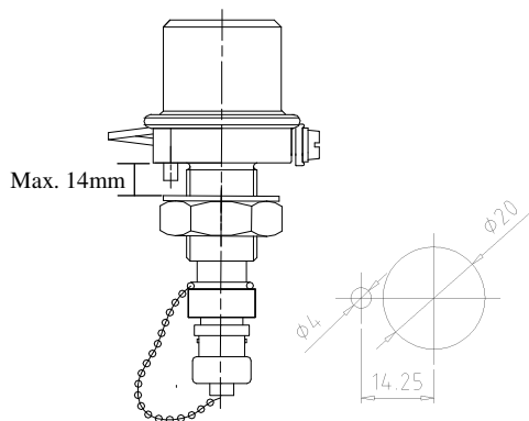
General Purpose bracket, for mounting hole Ø20mm
