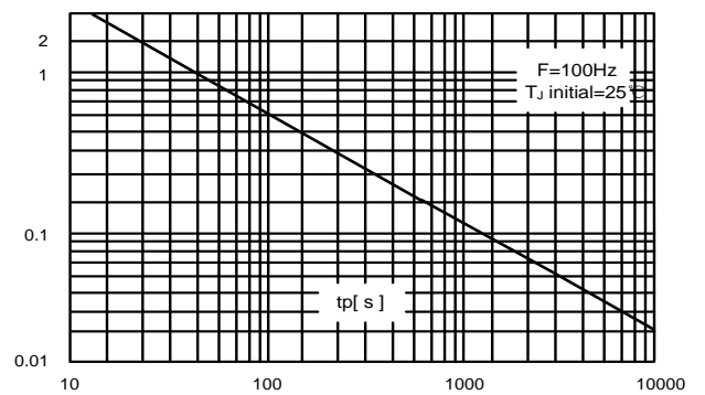
FIG.2-Peak pulse current versus pluse duration ( maximum values )
