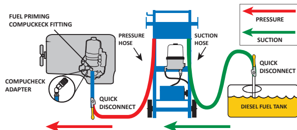
PRIMING WITH FILTRATION (NOTE: PACCAR MX ENGINES ARE PRIMED ON FUEL RETURN SIDE)
