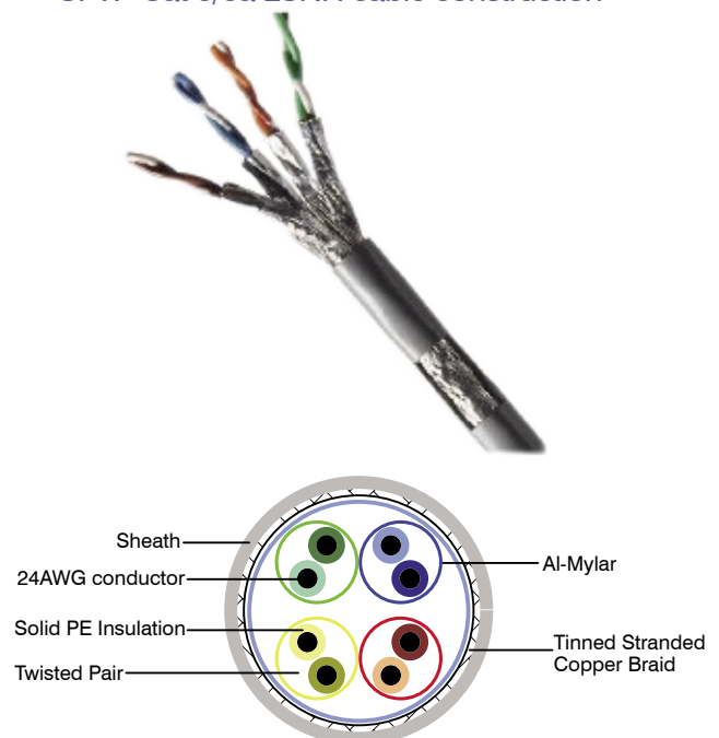
SFTP Cat 6/6a LSNH cable construction
