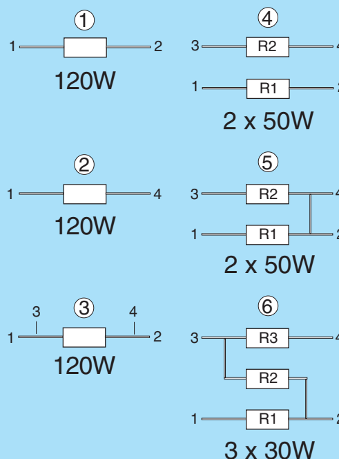
Version 5: ohmic value between contact 2 and 4 = 3 mΩ
