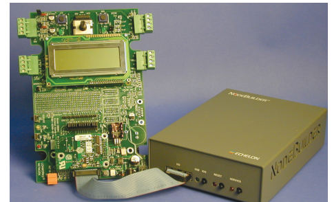
Gizmo 4 plugged into the LTM-10A Platform
