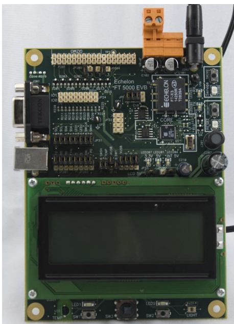
FT 5000 EVB Evaluation Board
