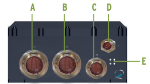
A: CPU I/O B: PMC & isolated GPI/GPO C: miniPCIe Slots I/O D: Power Supply E: 2x Monitoring & 2x User's LEDs
