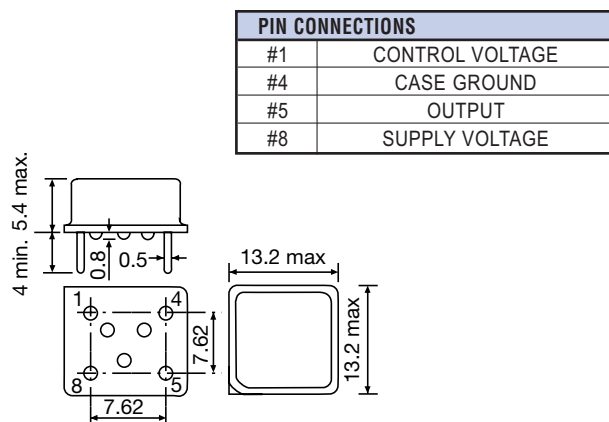
Figure 1) ECX-VXO-83X – Side, Bottom and Top views
