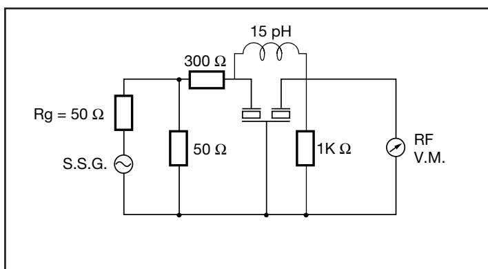
Figure 2) XT Series - Measuring Circuit
