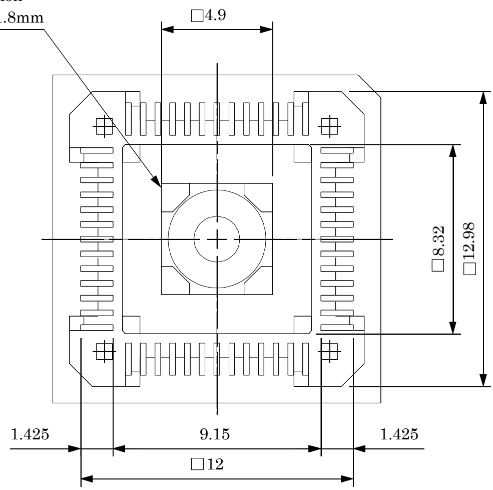
BOTTOM VIEW
