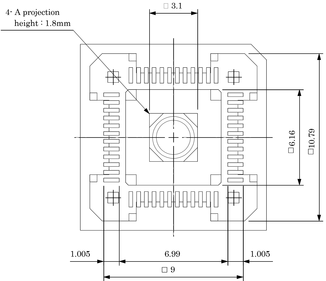
BOTTOM VIEW
