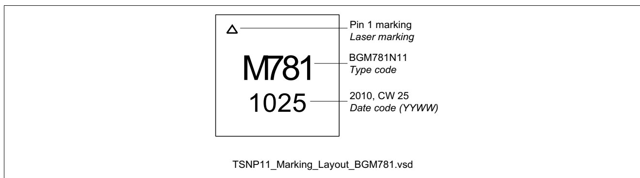
Figure 6 Marking layout
