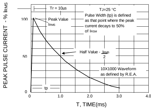
FIG.5 - PULSE WAVEFORM
