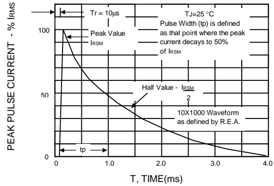
FIG.4 - PULSE RATING CURVE
