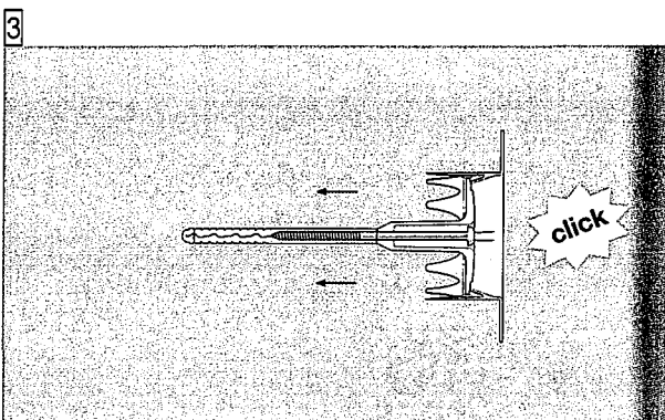
Assemble anchor and plate VT 2G
