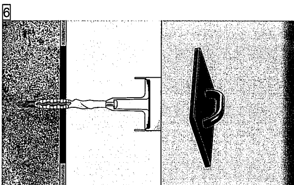
Insert the ejotherm STR cap with the help of a float
