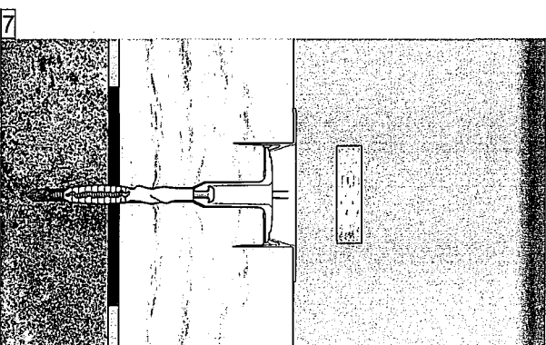
Insert the ejotherm STR cap
