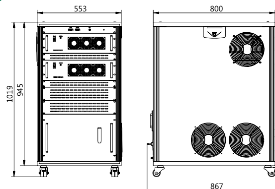
Atlantic 20-1064/532/355, Atlantic 40-1064/532/355, Atlantic 60-1064/532/355 power supply outline drawings
