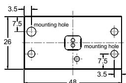
TK3 dimensions
