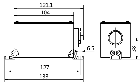
LightWire FFS200CHI laser isolator & collimator unit outline drawing
