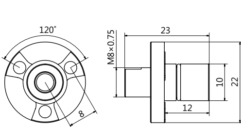
LightWire FFS10/100CHI laser collimator flange outline drawing
