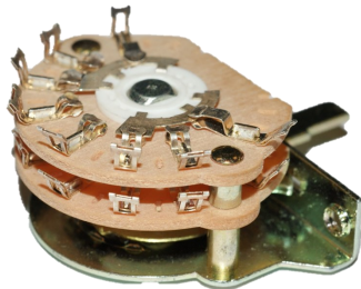
2-Deck, 4-Pole "Super Switch"
