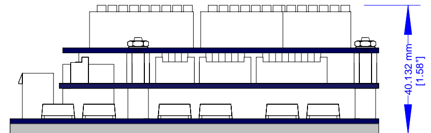
ACS Series Drive Assembly with Connector brd
