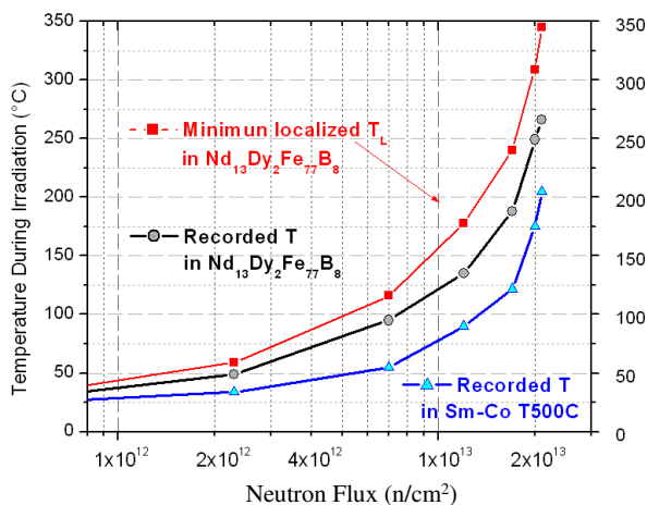
Figure 15. Recorded temperatures caused by thermal effect of radiation vs. neutron flux.
