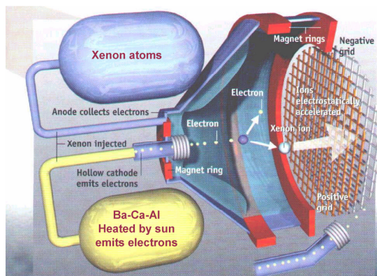
Fig. 1. Xenon ion propulsion engine with high temperature magnet used in Deep Space I 4
