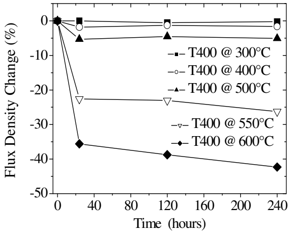
Figure 7. Magnetic flux change versus time at various temperatures under vacuum ( 10^{-5} Torr) for T400 UHT Sm-Co magnets.
