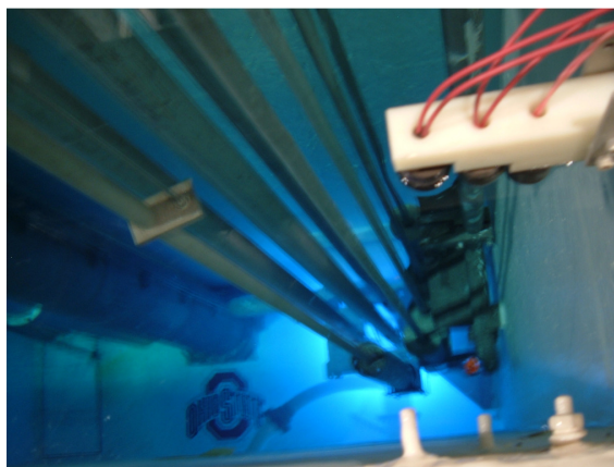
Figure 12: OSU Research Reactor at full power (450 kW) during the radiation experiment.
