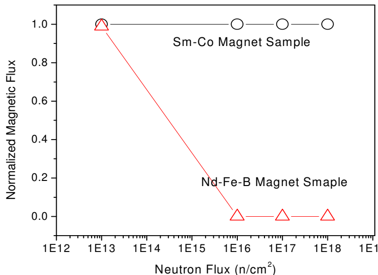
Figure 14. Normalized magnetic flux of permanent magnets versus neutron flux
