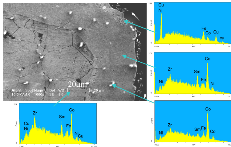
Figure 10. Microstructure and compositional analysis of the cross-section of T550 magnet after exposure to 700°C for 240 hours under a vacuum of 10^{-5} Torr
