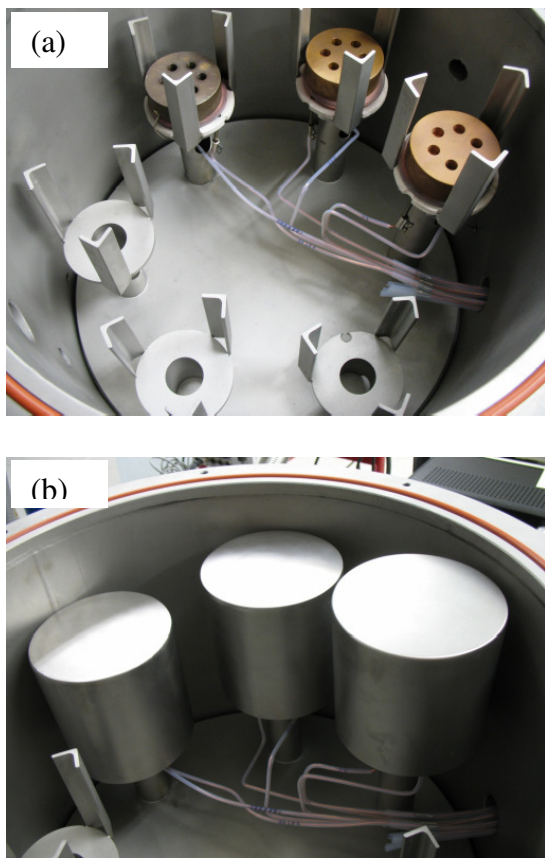
Figure 5: Top view of heater assembly inside the vacuum chamber (a), and final heaters assembly showing oxygen-free copper plates with lids inside the vacuum chamber (b). The lids protect the magnets and collect out-gassed material so that it does not coat the chamber wall.
