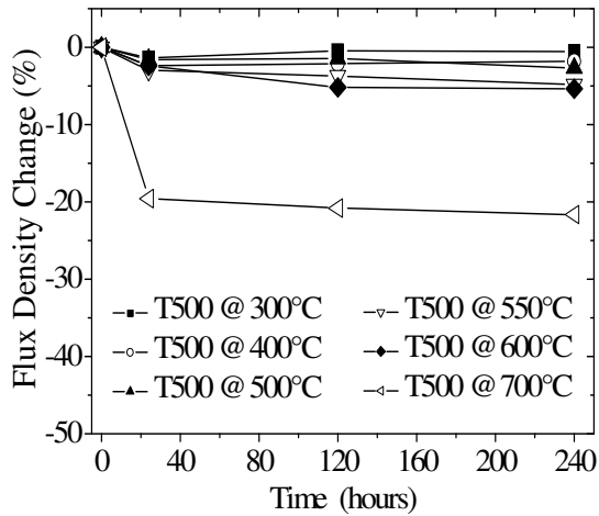
Figure 8. Magnetic flux change versus time at various temperatures under vacuum ( 10^{-5} Torr) for T500 UHT Sm-Co magnets.
