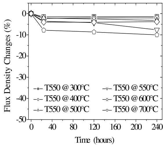
Figure 9. Magnetic flux change versus time at various temperatures under vacuum ( 10^{-5} Torr) for T550 UHT Sm-Co magnets.
