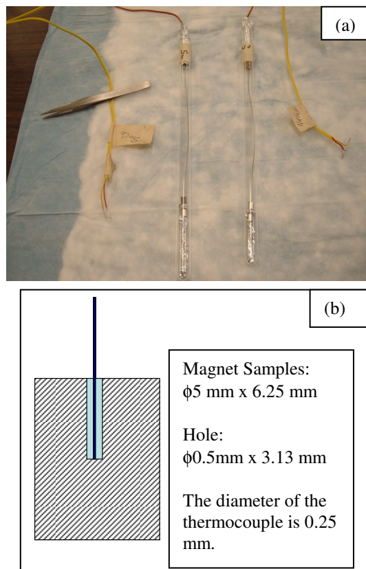
Figure 13: Magnet samples, thermocouples and quartz tubes for the irradiation experiments (a) Picture showing sample and thermocouple assembly and (b) sketch showing the position of thermocouple inside the sample.
