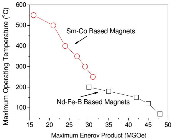
Figure 2. Maximum energy product versus maximum operating temperature for rare earth permanent magnets
