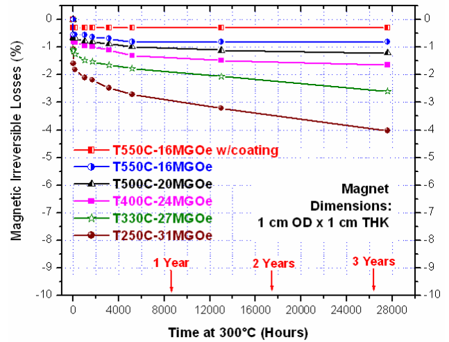
Figure 3. Thermal stability of various Sm-Co magnets at 300°C in air for more than three years
