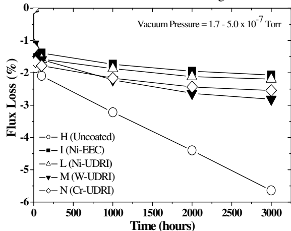
Figure 11. Average flux loss for T500C magnets at 400°C in vacuum
