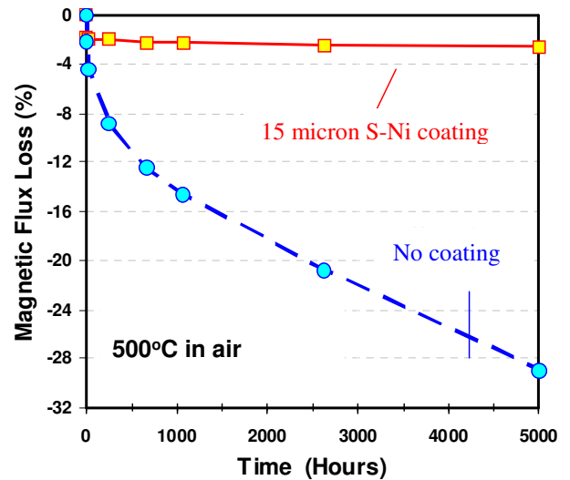
Figure 4. Magnetic flux loss for SmCo T500 magnets at 500°C in air for 5000 hours
