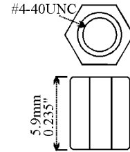
3806 Threaded Bushing
