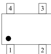
SC-82AB(TOP VIEW)
