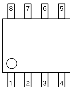
SOP-8(TOP VIEW)
