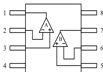
SOP-8(TOP VIEW)
