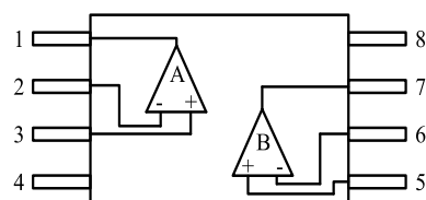
TSSOP-8(TOP VIEW)
