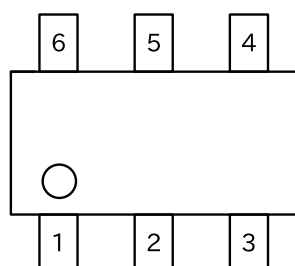
SOT-26(TOP VIEW)
