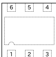
VSON6-2x2(TOP VIEW)
