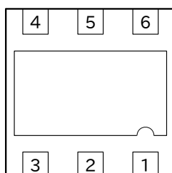
VSON6-2x2(BOTTOM VIEW)
