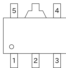
SOT-89-5(TOP VIEW)
